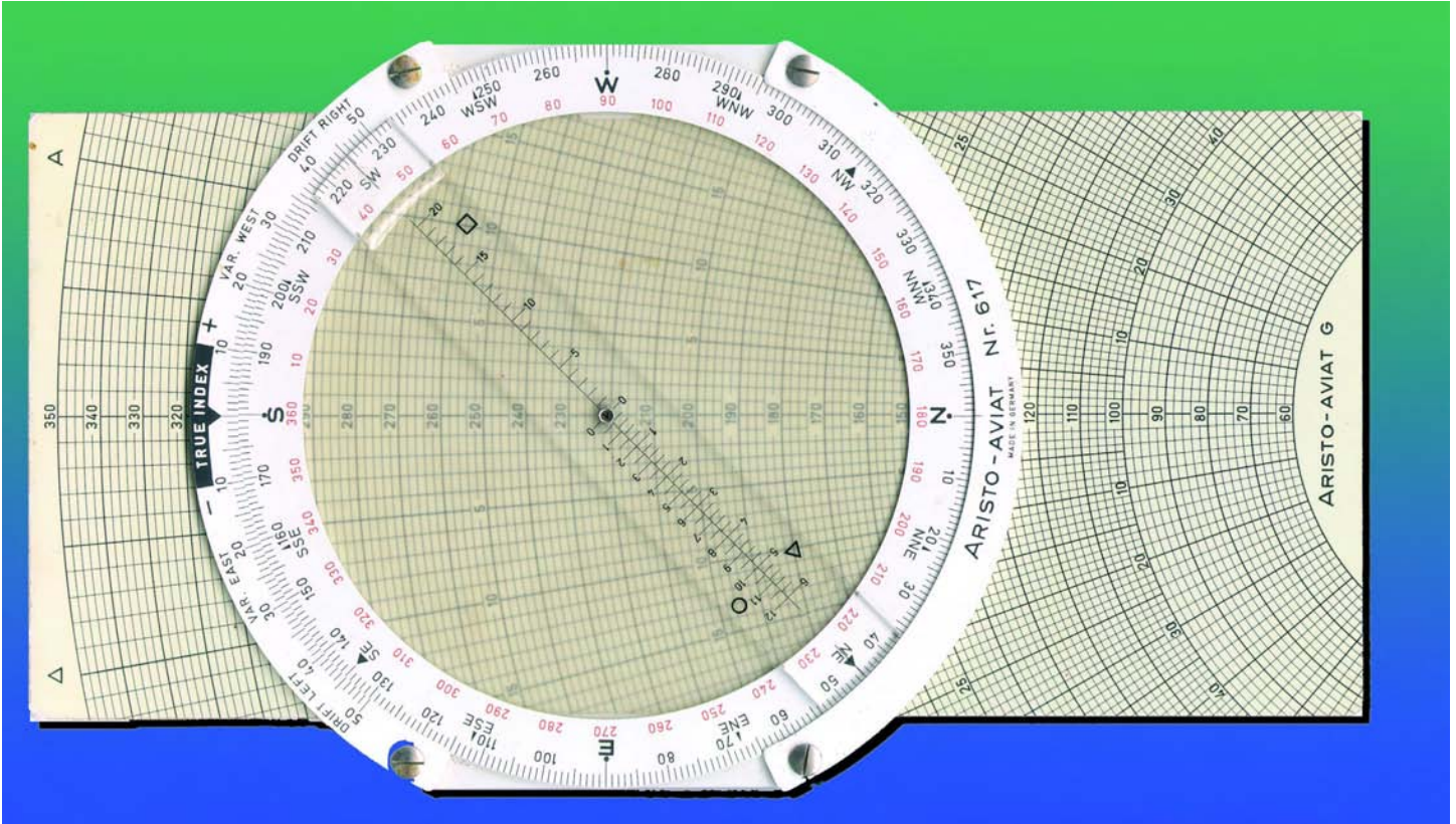
ARISTO 617 AVIAT, METAL AND PLASTIC, GERMANY, OPPOSITE VIEW.
